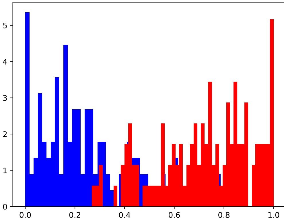
RHI
